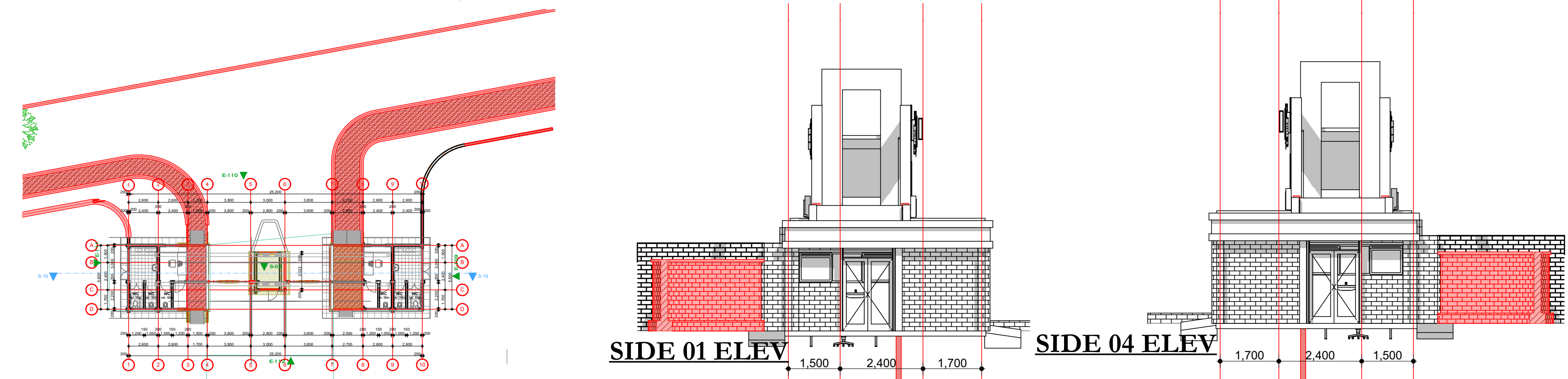
FLOOR PLAN
