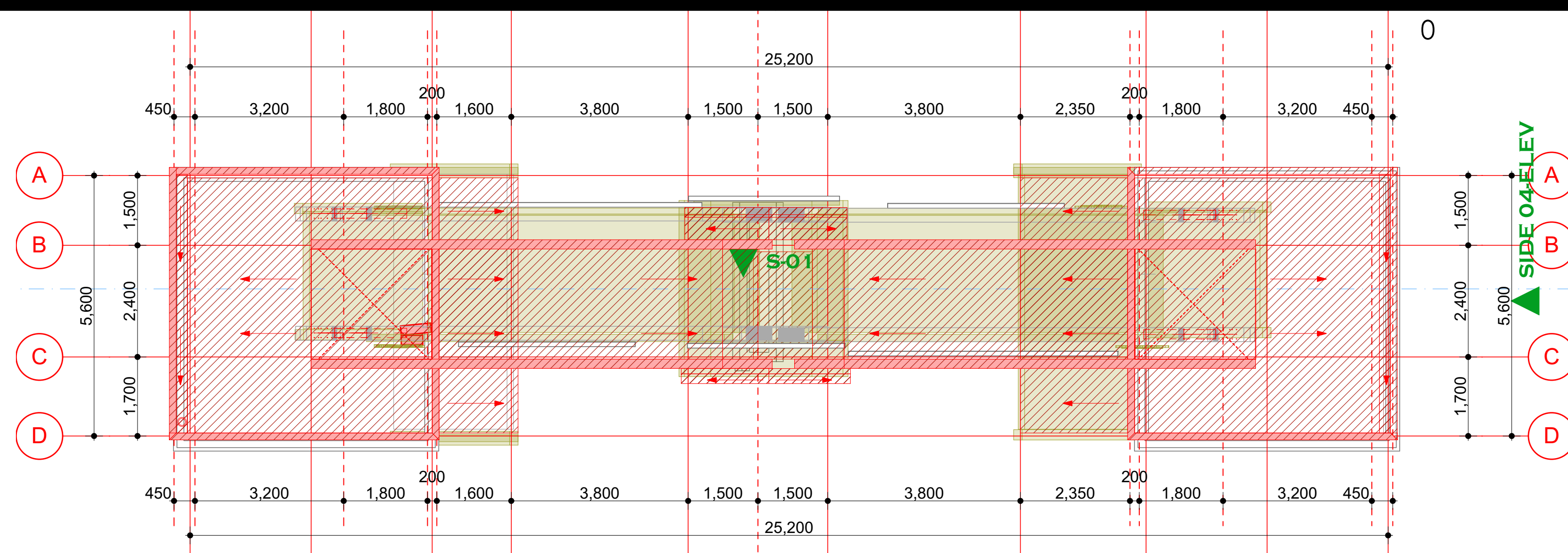
ROOF PLAN
