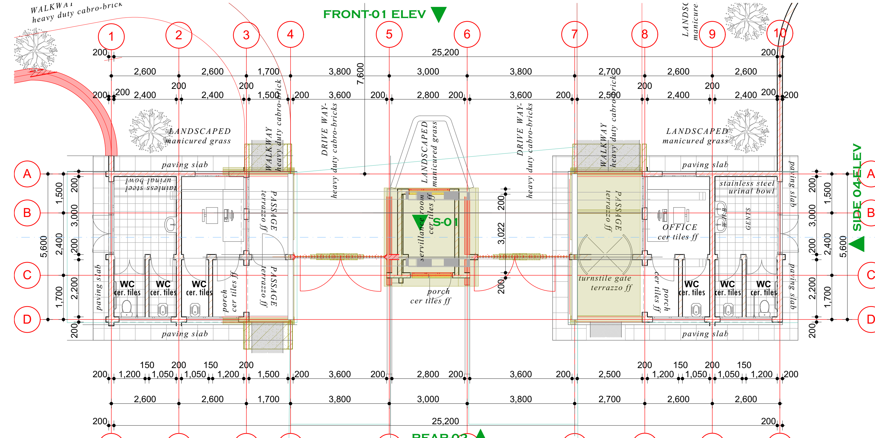
FLOOR PLAN
